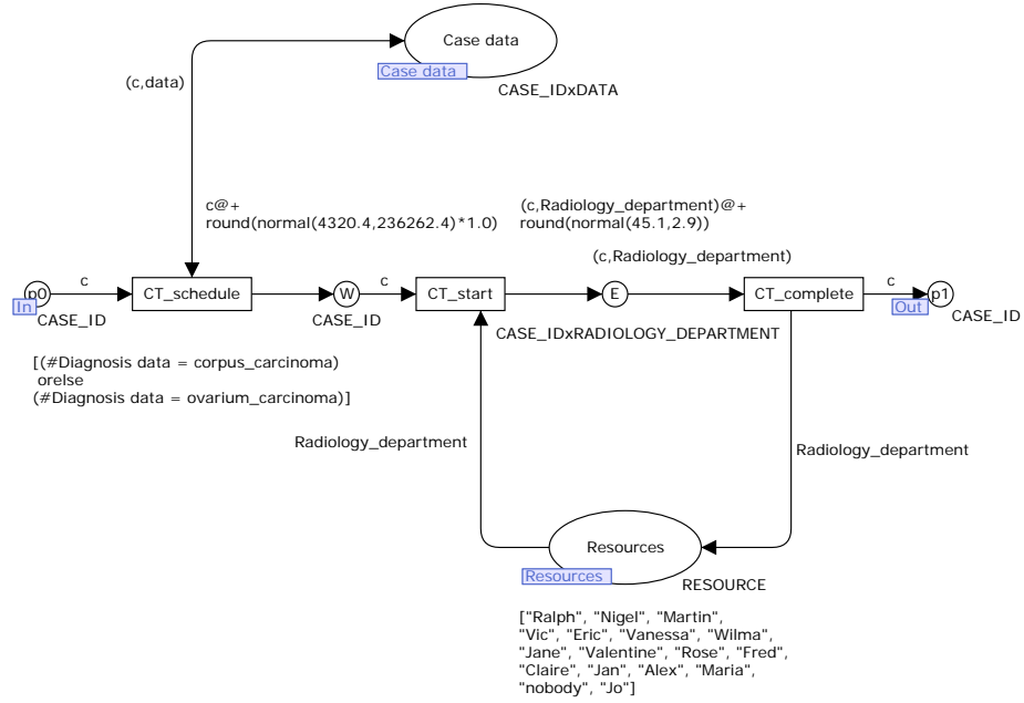
Fig. 10. Sub-page for the “CT” activity, showing how the simulation information related to the “CT” activity is represented in the CPN model
