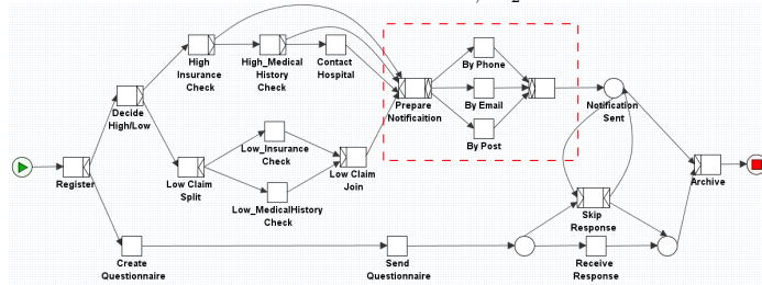
c. Model, M_3
