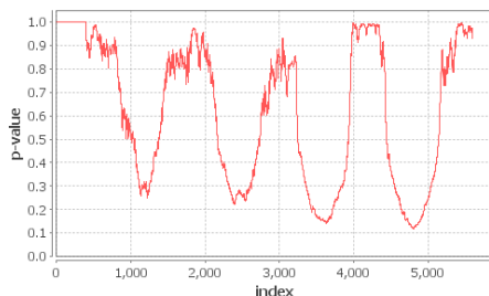
Fig. 7. Average significance probability (over all activity pairs) of KS -test on J -measure estimated for each trace. X-axis represents the trace index. Y-axis represents the significance probability of the test. Troughs signify change points.
