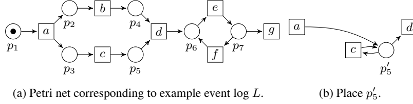
Fig. 3: A Petri net corresponding to event log L , discoverable by the ILP-based process discovery algorithm (3a) and an alternative place p'_5 for place p_5 given L' (3b).
