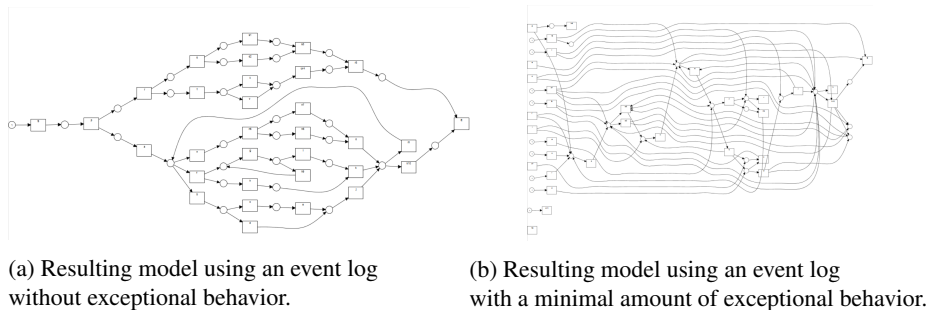
Fig. 2: Discovered Petri nets after applying conventional ILP-based process discovery on event logs with and without the presence of exceptional behavior in the event log.
