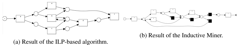
Fig. 1: Process discovery results of the conventional ILP-based discovery and the Inductive Miner [4] based on a log consisting of milestone pattern based behavior.
